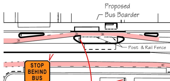
Figure 2: Second bus boarder layout
